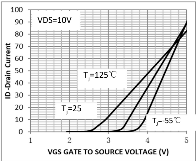
Figure 8. Transfer Characteristics
