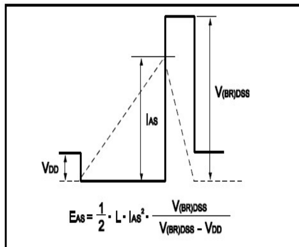
Fig.18 Avalanche Waveform
